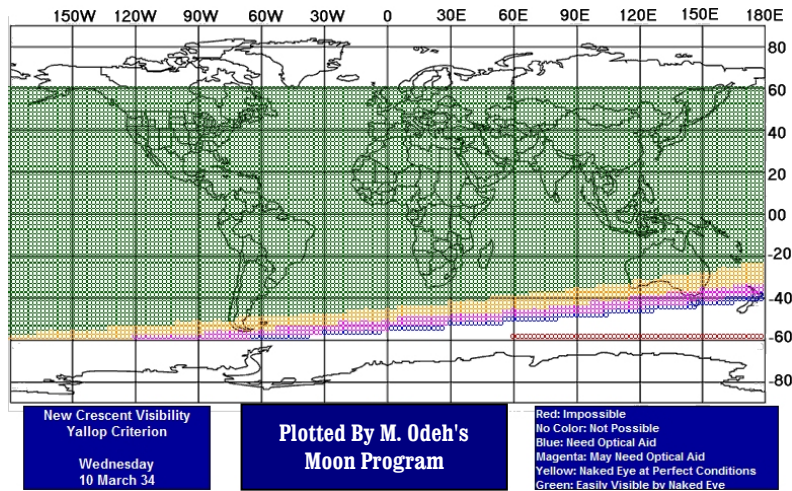
Figure 62: Nisan 1 Visibility Plot for AD 34
